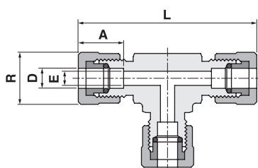
Union Tee
