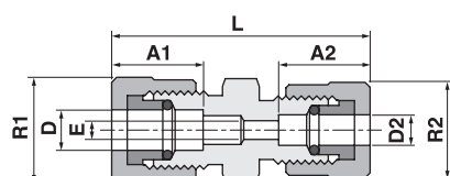
Reducing Union
