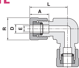
Union Elbow
